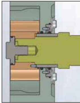
Double-O-Ring Seal
