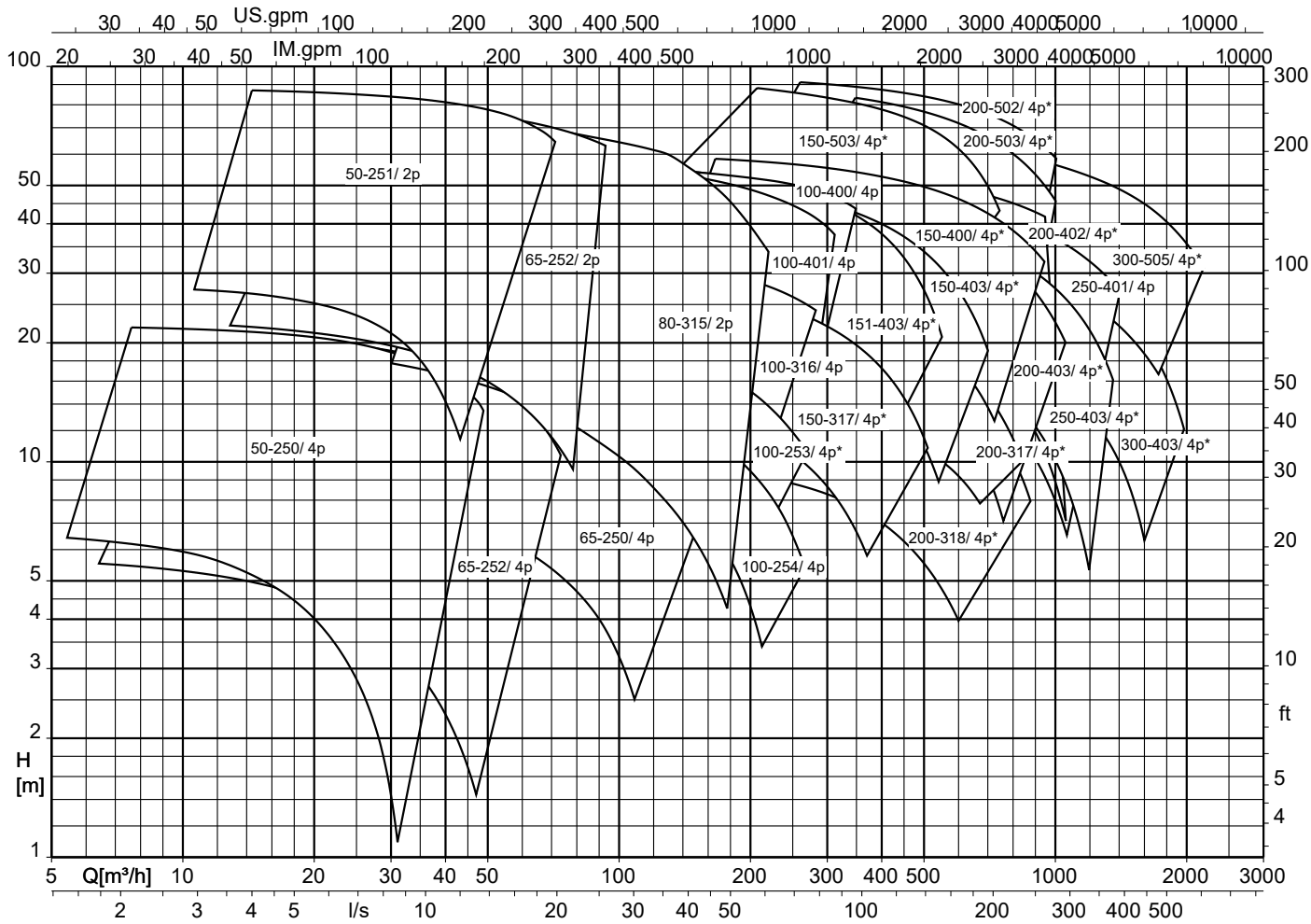
Sewatec/Sewabloc K + *K-max, n = 2900/1450 rpm (diameter-based selection chart)
