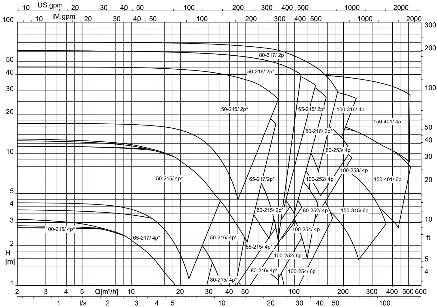
Sewatec/Sewabloc F + *F-max, n = 2900/1450/960 rpm (diameter-based selection chart)
