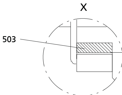
Fig. 9: Detail X: impeller wear ring of K impeller
