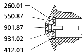
Fig. 11: Impeller fastening for bearing brackets S06, S07 and S08, except Sewatec size 500-632
