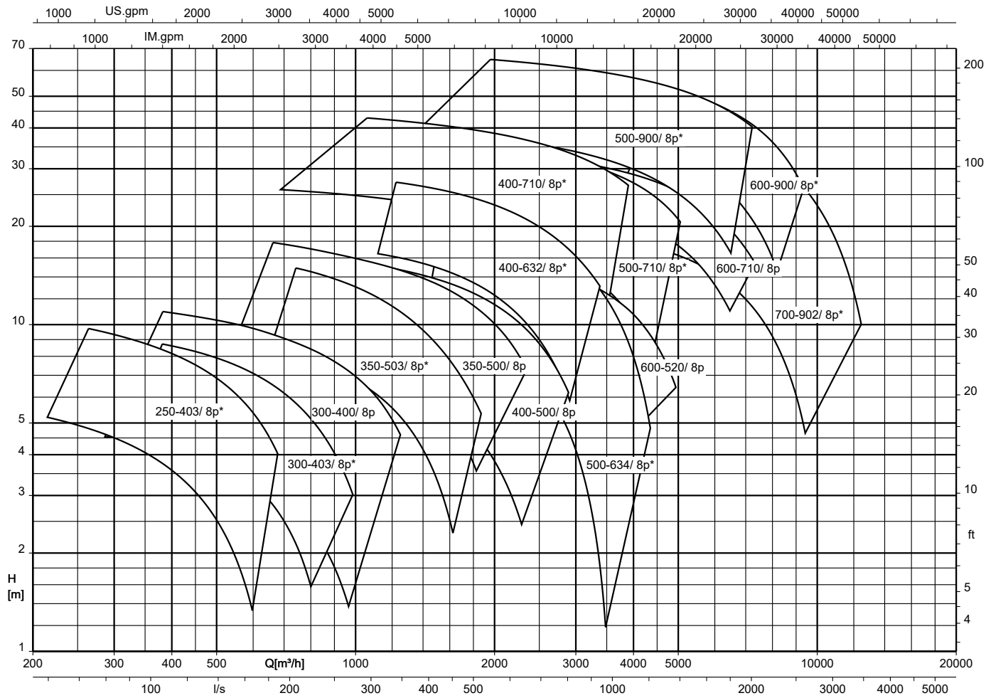
Sewatec/Sewabloc K + *K-max, n = 725 rpm (diameter-based selection chart)
