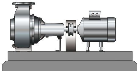
Pump set with directly coupled drive, baseplate, coupling (also with coupling spacer), coupling guard and height adjustment of the motor
