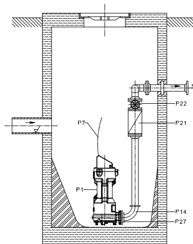
Suggested installation layout 2
