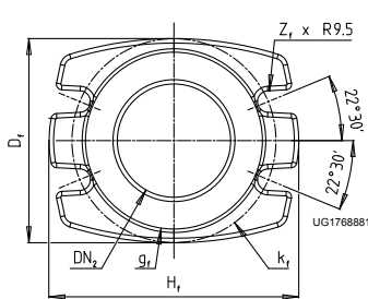
Pump flange DN 80 / 100
