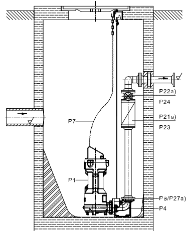
Suggested installation layout 3
