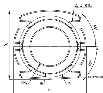
Pump flange DN 150
