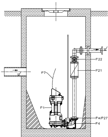
Suggested installation layout 1
