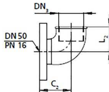
Connection elbow with internal thread and external thread (P14) and threaded flange (P27)
