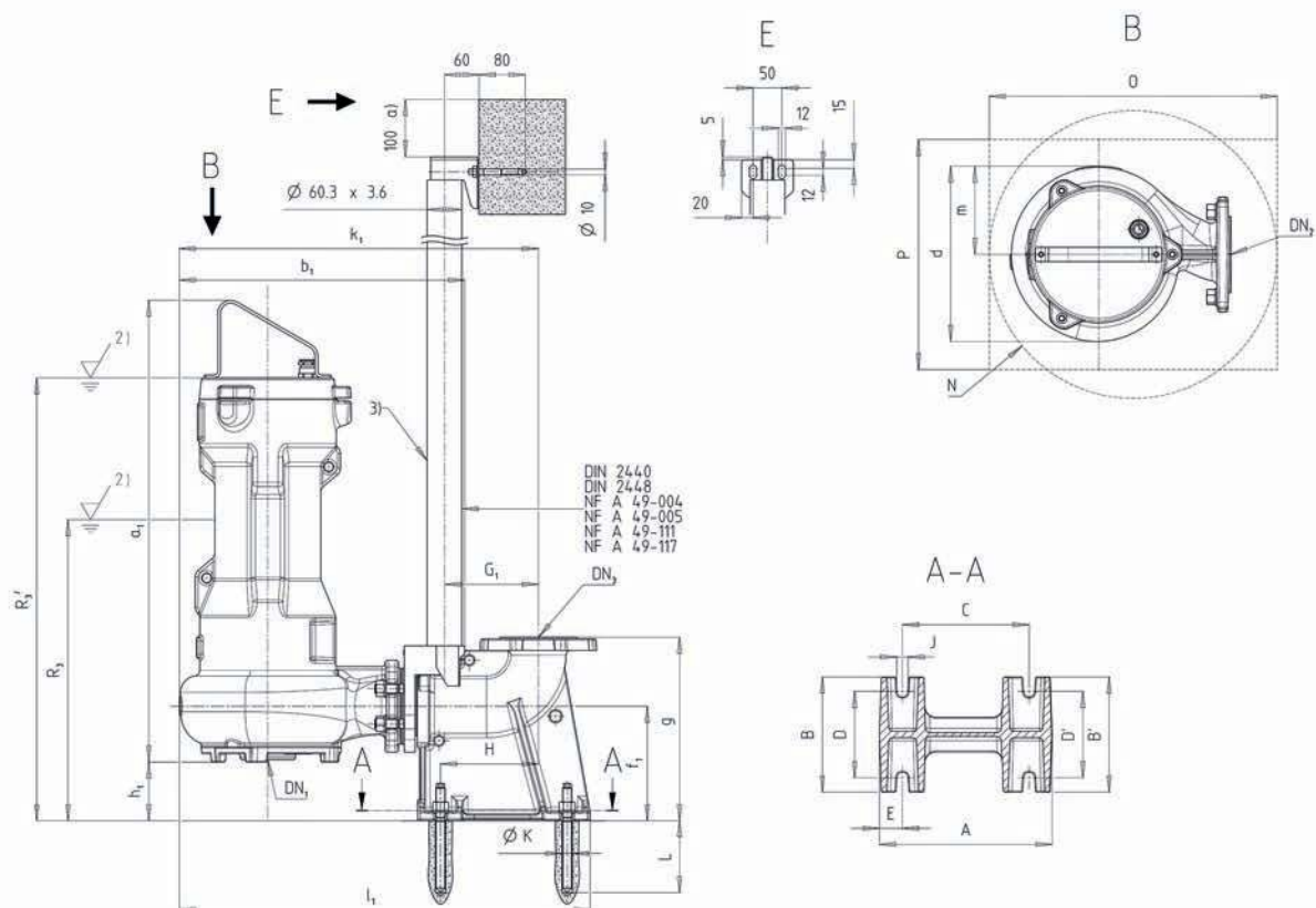
Fig. 8: Amarex 80, stationary installation, single guide rail arrangement
