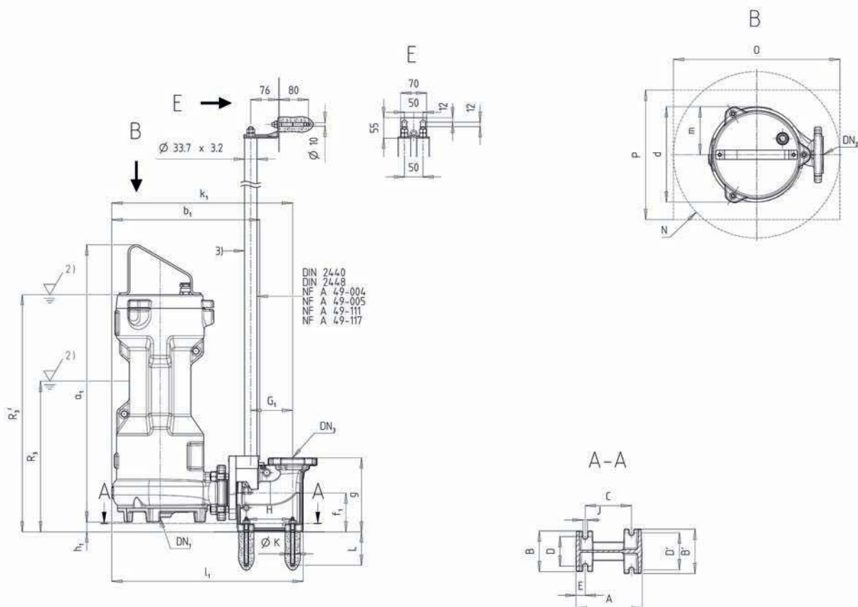
Fig. 4: Amarex 50, stationary installation, twin guide rail arrangement
