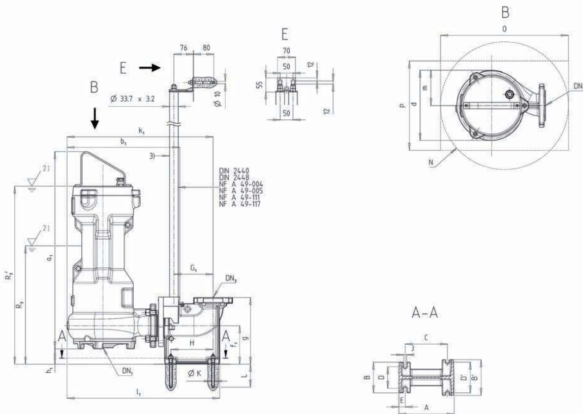
Fig. 6: Amarex 65, stationary installation, twin guide rail arrangement
